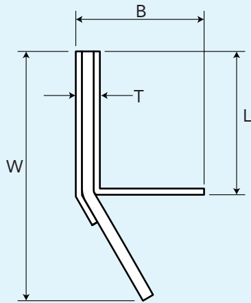
Lip Seal
